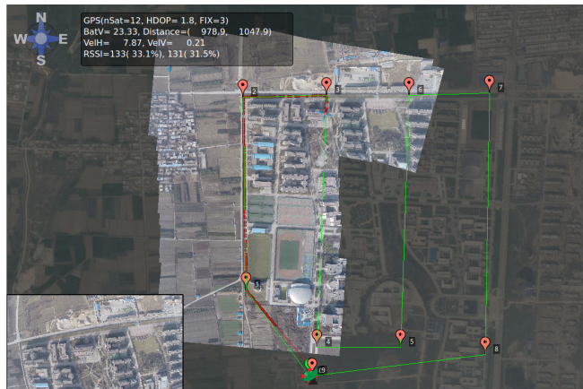
Fig. 1. We integrate Map2DFusion into the self-developed ground control station, where the orthoimage is generated and visualized online during the flight. The figure shows that the orthoimage is well aligned to Bing satellite map automatically after GPS trajectory fitted.
