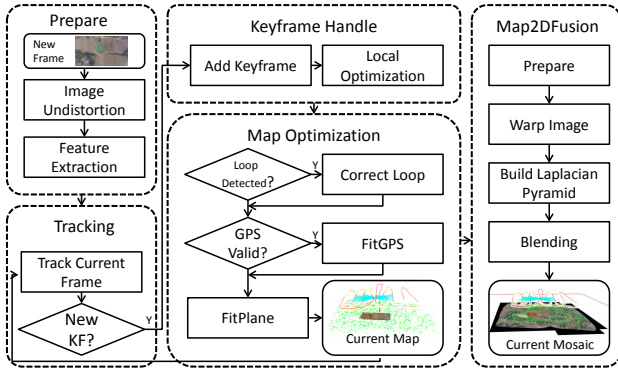
Fig. 2. The framework overview of our system.
